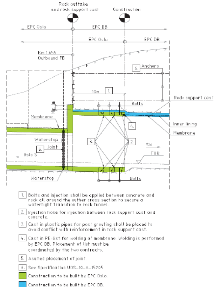
Fig 4: Principles for the transition between concrete and rock tunnel
